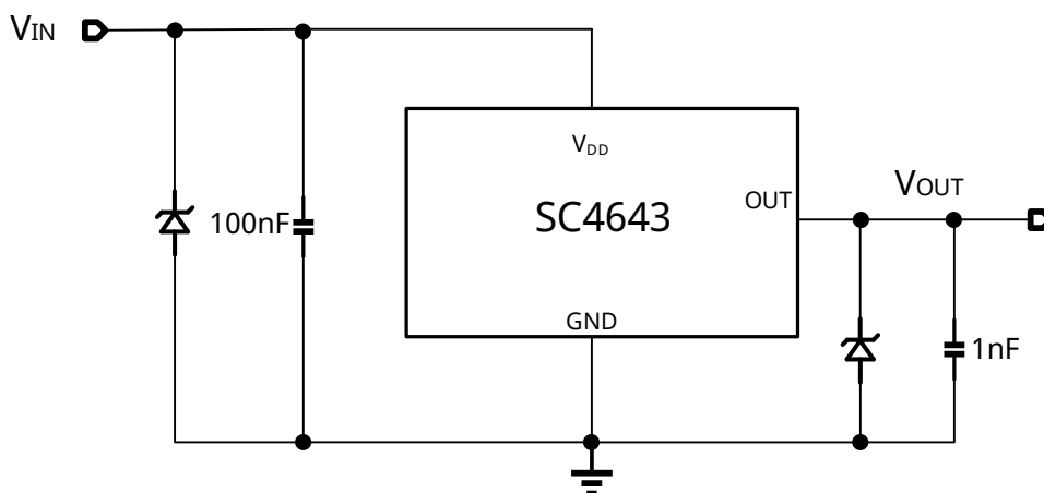
Fig.7 TO92U Typical Application Schematic
