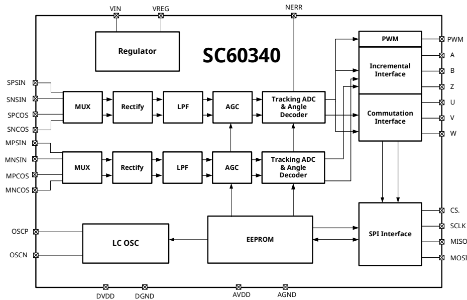
Fig.3 Block Diagram
