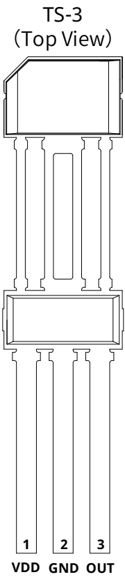
Fig.2 Pin Description
