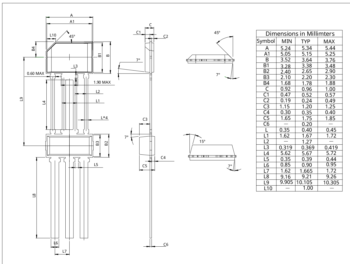
Fig.8 Package Dimension
