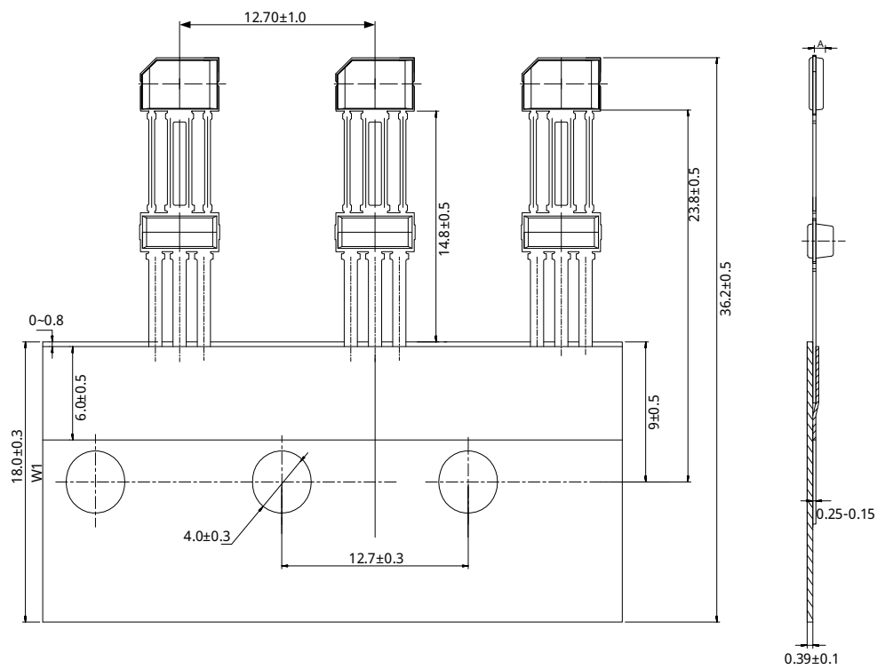
Fig.9 Packing Dimension
