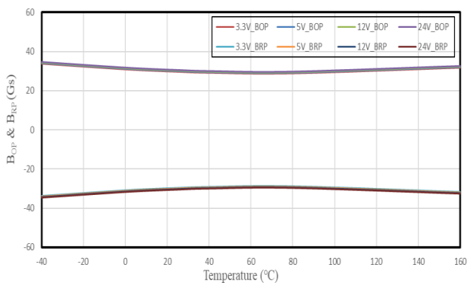
SC2443 B_{OP} & B_{RP} VS. Temperature
