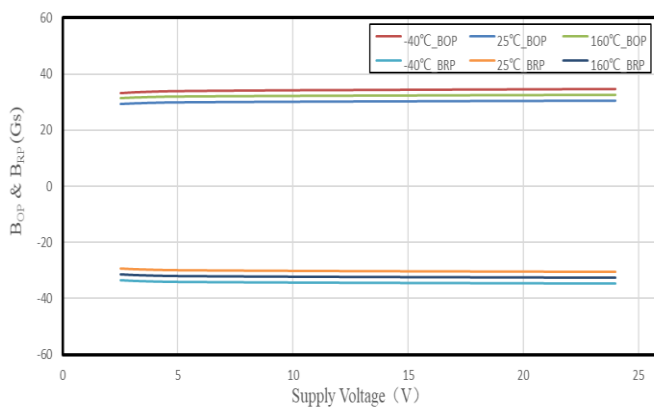
SC2443 B_{OP} & B_{RP} VS. Supply Voltage
