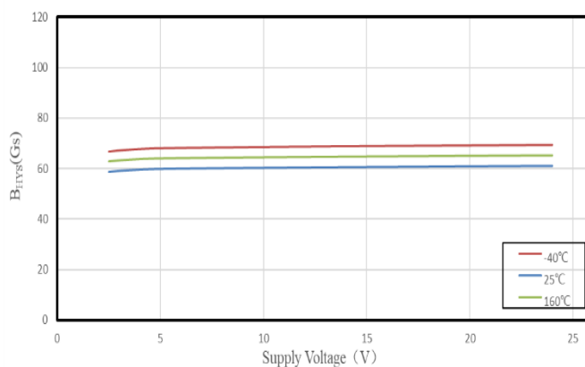
SC2443 B_{HYS} VS. Supply Voltage
