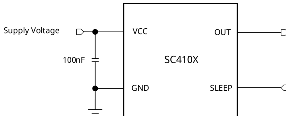
Fig.7 Typical Application Circuit
