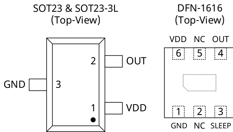
Fig.2 SOT23 & SOT23-3L(Left) and DFN1616(Right)Pin Description
