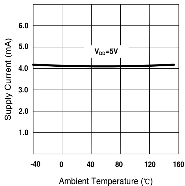
I_{DD} vs T_A
