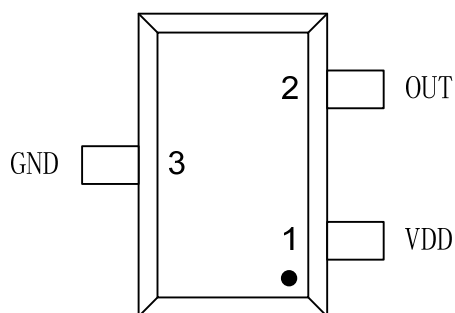
3-Terminal SOT-23 S0 Package (Top View)
