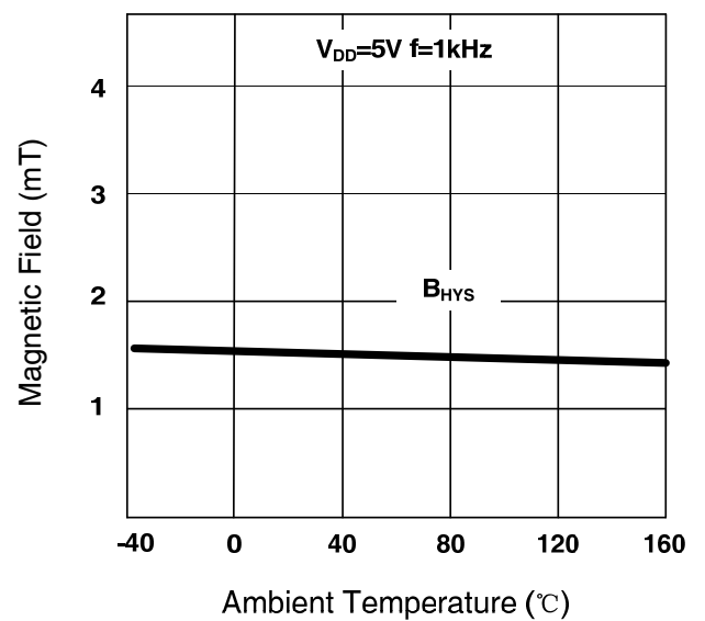
SC2436 B HYS vs T A
