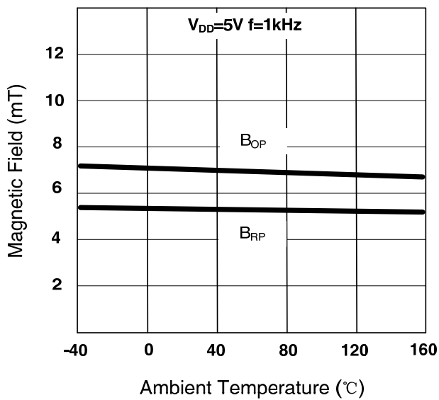
SC2434 B OP and B RP vs T A
