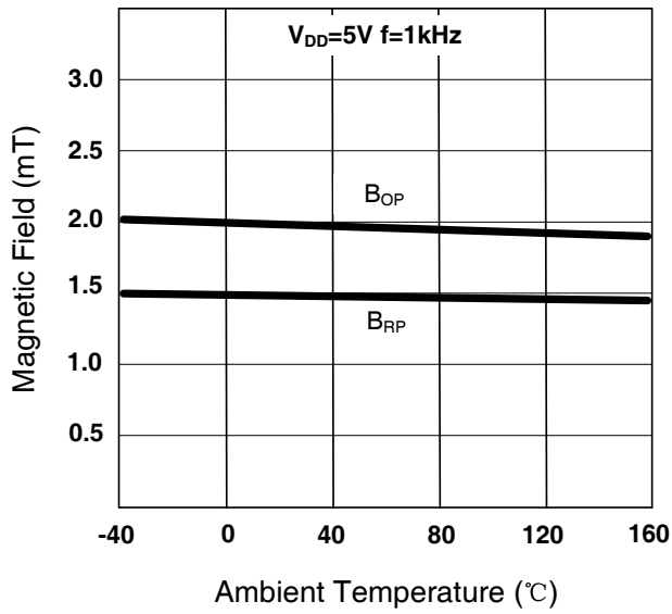
SC2430 B_{OP} and B_{RP} vs T_A
