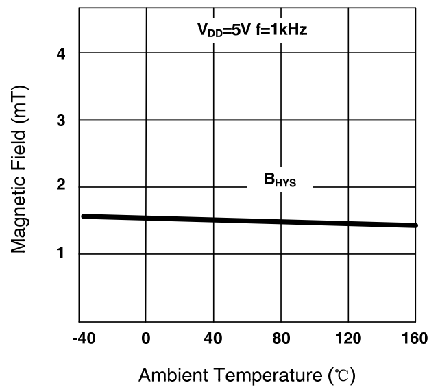
SC2434 B HYS vs T A
