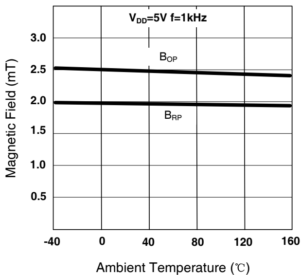
SC2432 B_{OP} and B_{RP} vs T_A
