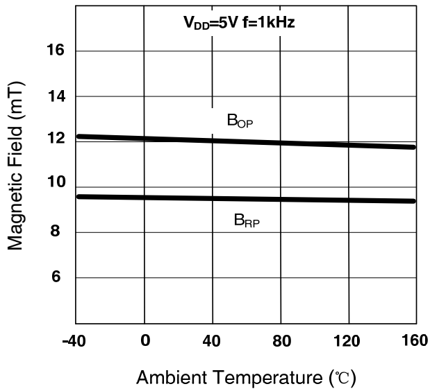
SC2438 B_{OP} and B_{RP} vs T_A
