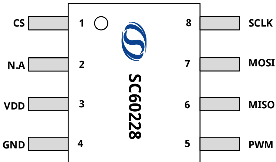
Fig.4 SC60228 Terminal Configuration
