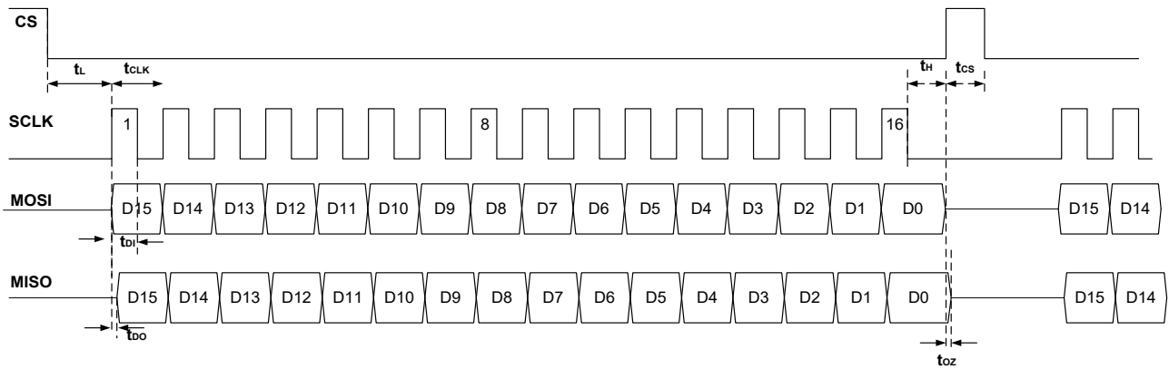
Fig.8 SPI register read-write mode diagram
