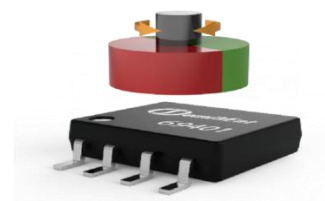
Fig.1 Installation diagram
