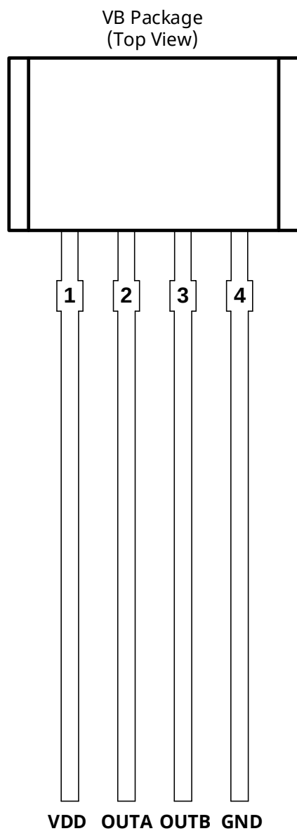
Fig.2 Pin Description
