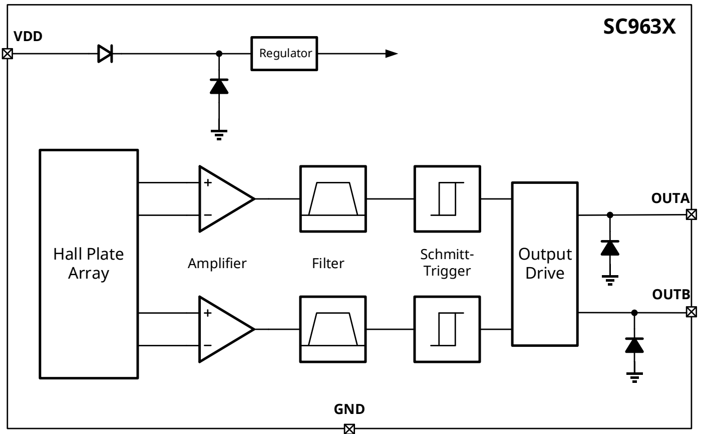
Fig.7 Block Diagram
