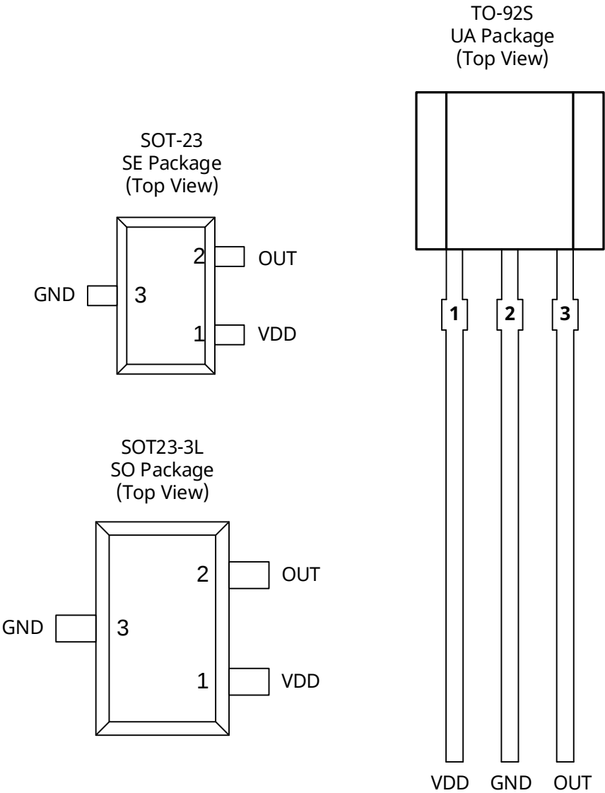
Fig.2 Terminal Configuration
