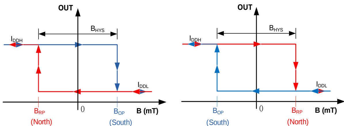
Fig.5 Transmission curve graph
