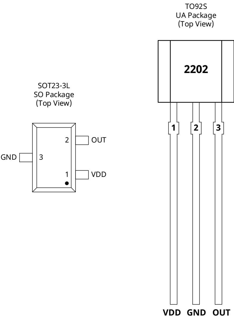
Fig. 2: Terminal Configuration
