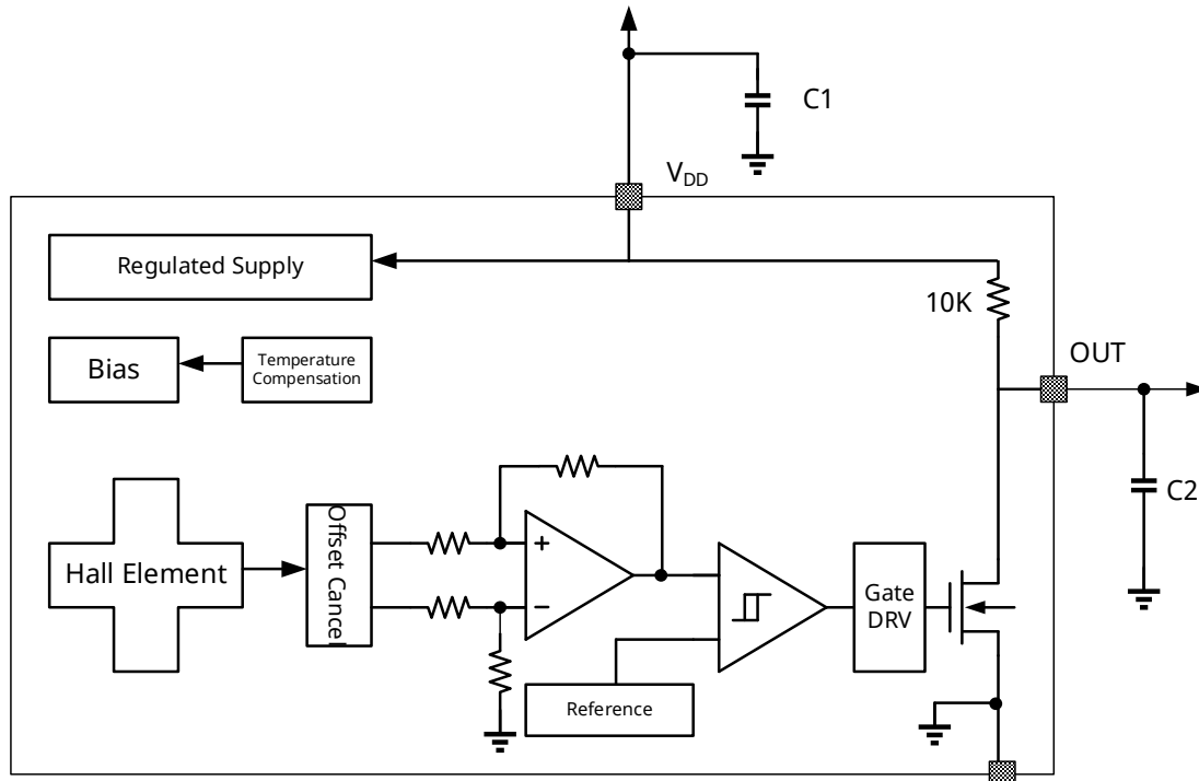
Fig. 3: Function Block Diagram
