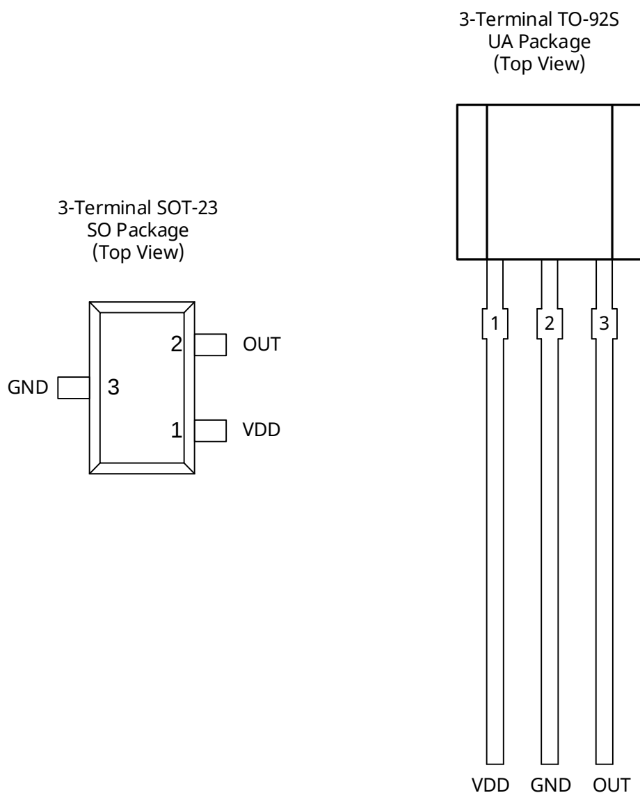
Fig.2 Terminal Configuration
