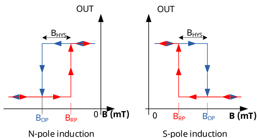
Fig.5 Magnetic Transfer Function
