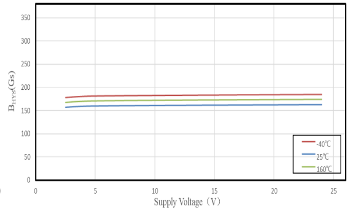
SC2448 B HYS VS. Supply Voltage
