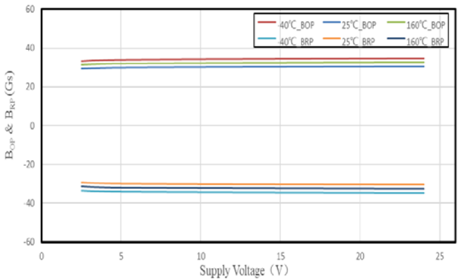
SC2443 B OP & B RP VS. Supply Voltage
