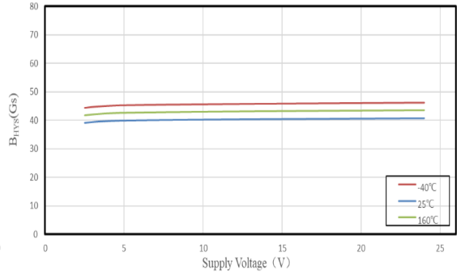
SC2442 B HYS VS. Supply Voltage
