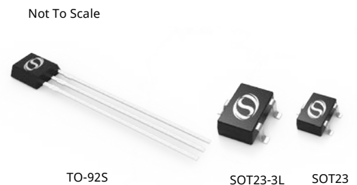
Fig.1 Package Outline
