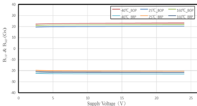
SC2442 B_{OP} & B_{RP} VS. Supply Voltage
