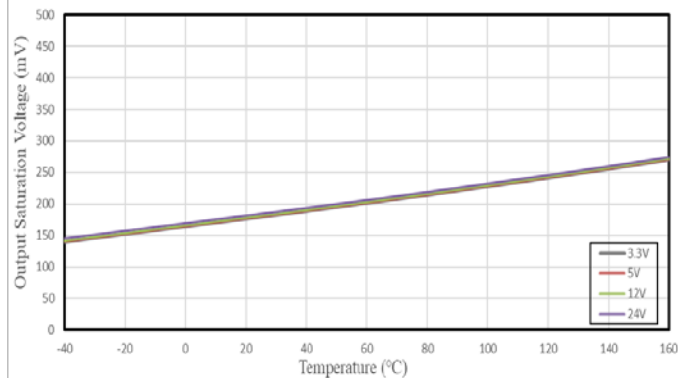
Output Saturation Voltage VS. Temperature
