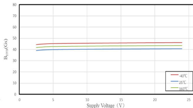
SC2442 B_{HYS} VS. Supply Voltage
