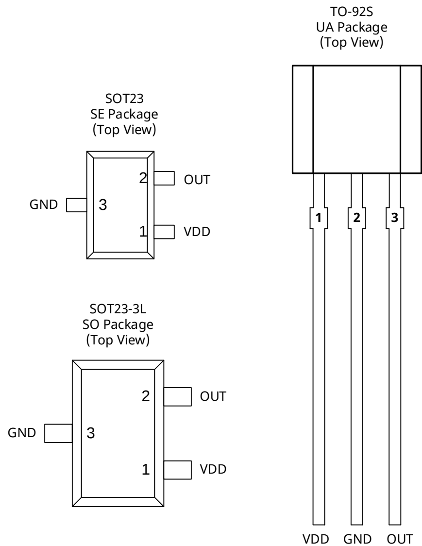
Fig.2 Terminal Configuration
