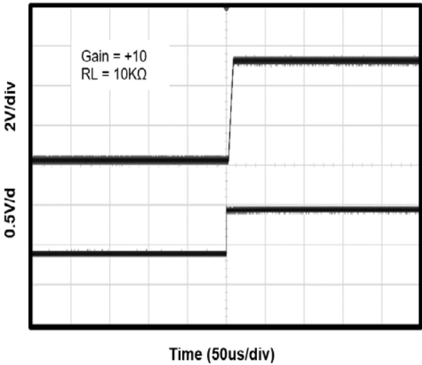
Figure 13. Negative Over-Voltage Recovery
