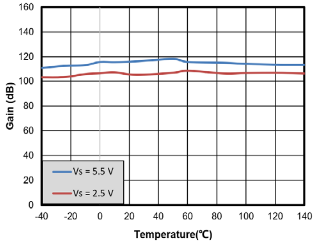
Figure 16. Open-Loop Gain vs. Temperature
