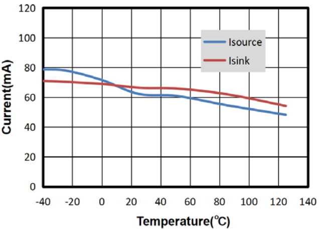
Figure 4. Short Circuit Current vs. Temperature
