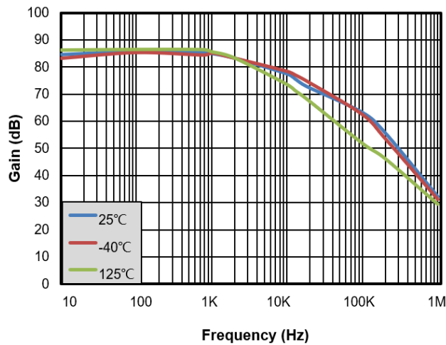
Figure 7. CMRR vs. Frequency
