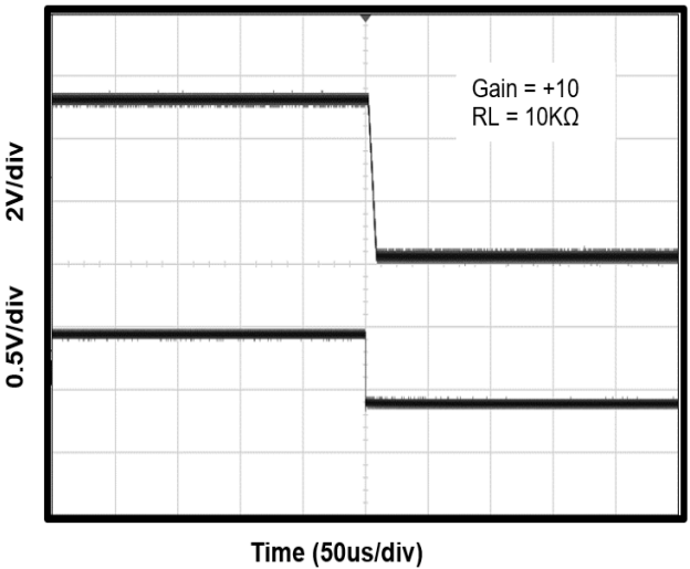
Figure 14. Positive Over-Voltage Recovery
