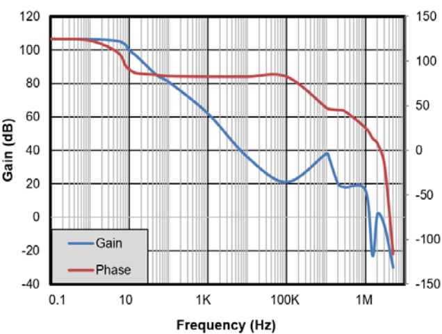
Figure 2. Open-Loop Gain and Phase
