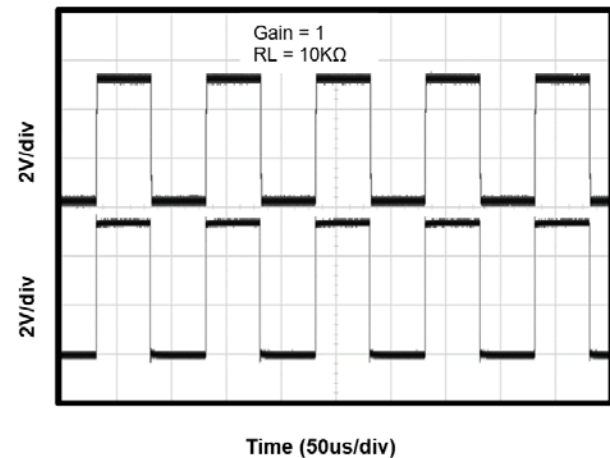
Figure 12. Large-Scale Step Response
